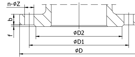
ASME B16.5 300LB Flanges
