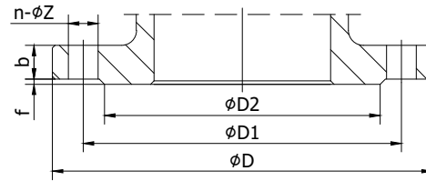
ASME B16.5 150LB Flanges
